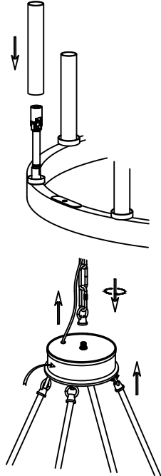
Connect side hanging rods to the wheel and wiring chamber.
