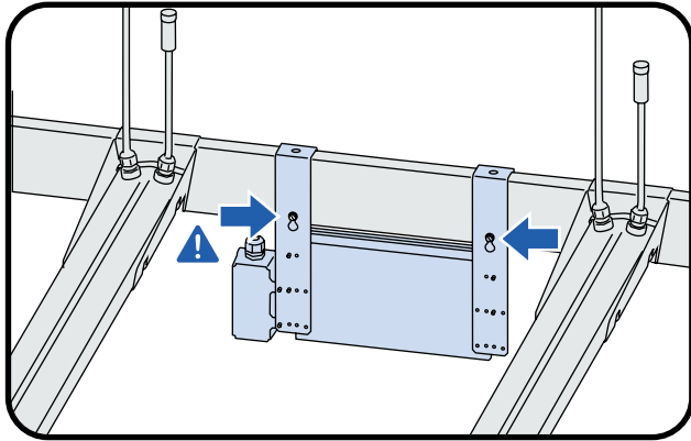
VAFS 2 LED Driver Mounting Option A Installation
