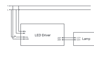
Push Dimming Connection using a Dali Driver
