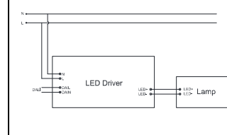
Dali Dimming Connection
