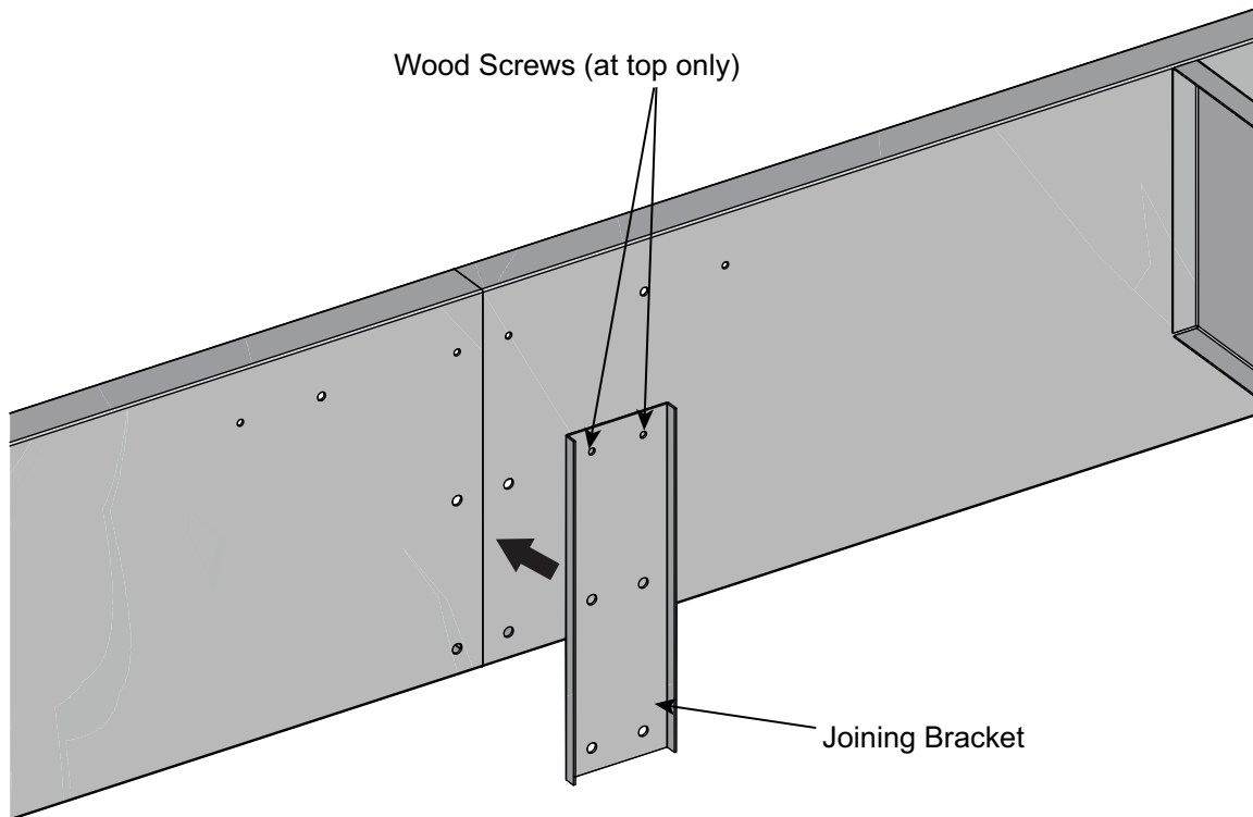
Fig. 10 – Joining Bracket
