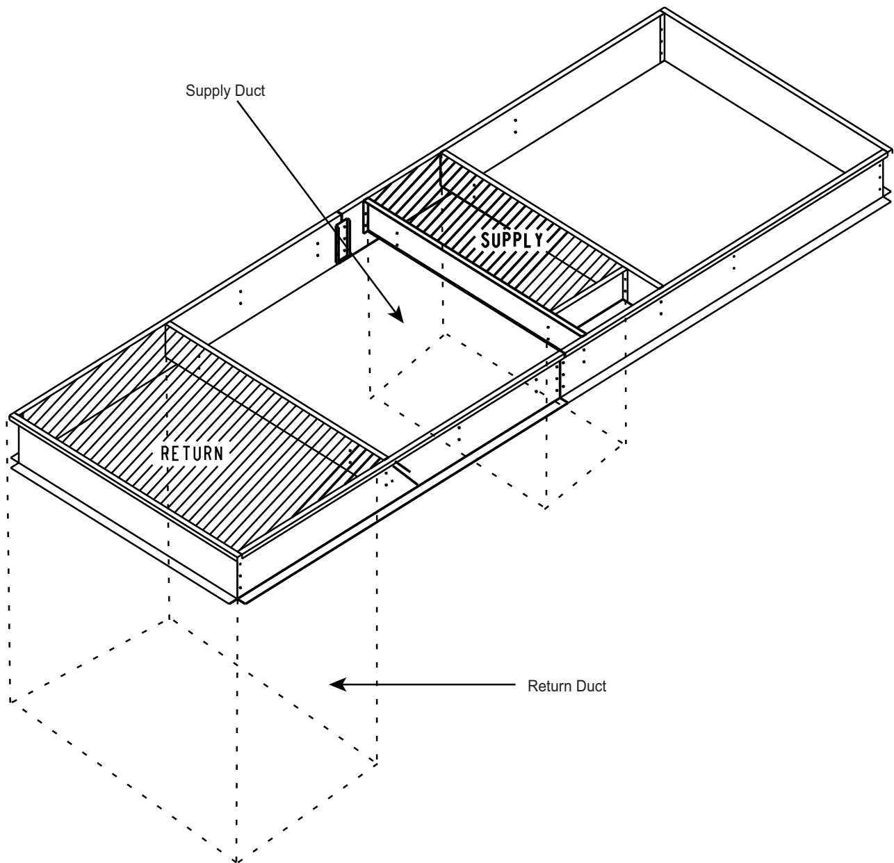
Fig. 13 — Attaching Ductwork
