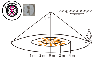
With Corridor Lens Mask: \phi 4-5m at 3m height
