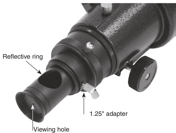
Figure 6-1. The collimating tool in the StarSeeker 100 focuser.
