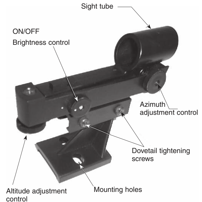
Figure 2-4. The Star Pointer finderscope with bracket
