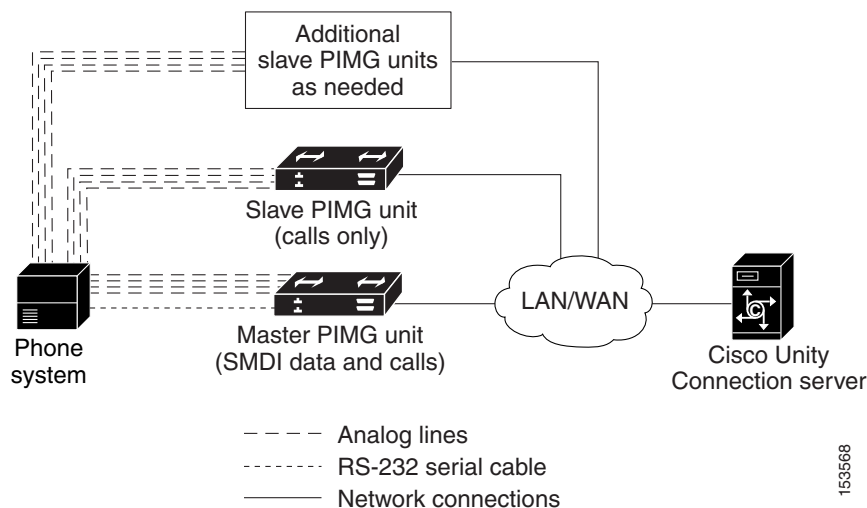
Figure 11-4 Connections for a Serial (SMDI, MCI, or MD-110) Integration Using Analog PIMG Units
