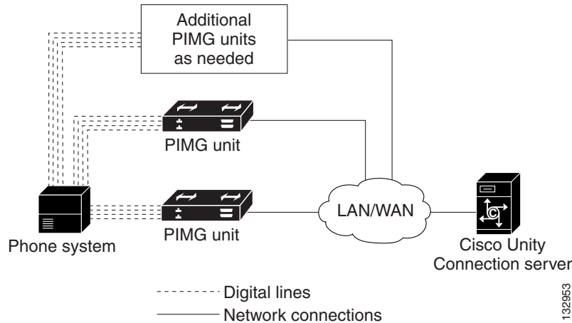
Figure 11-2 Connections for a Digital Integration Using Digital PIMG Units
