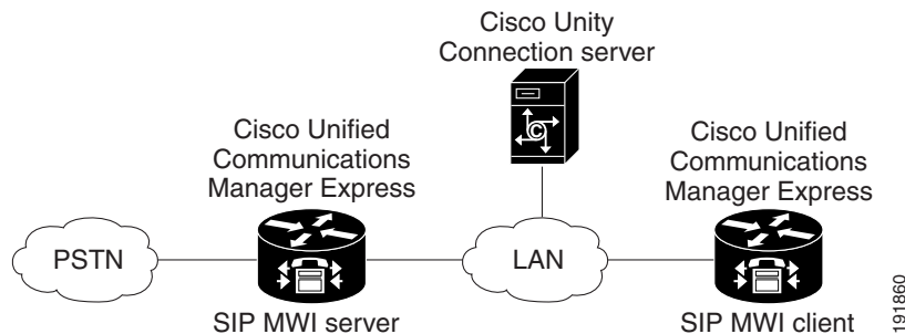
Figure 11-9 Connections between Multiple Cisco Unified CM Express Routers and a Single Cisco Unity Connection Server
