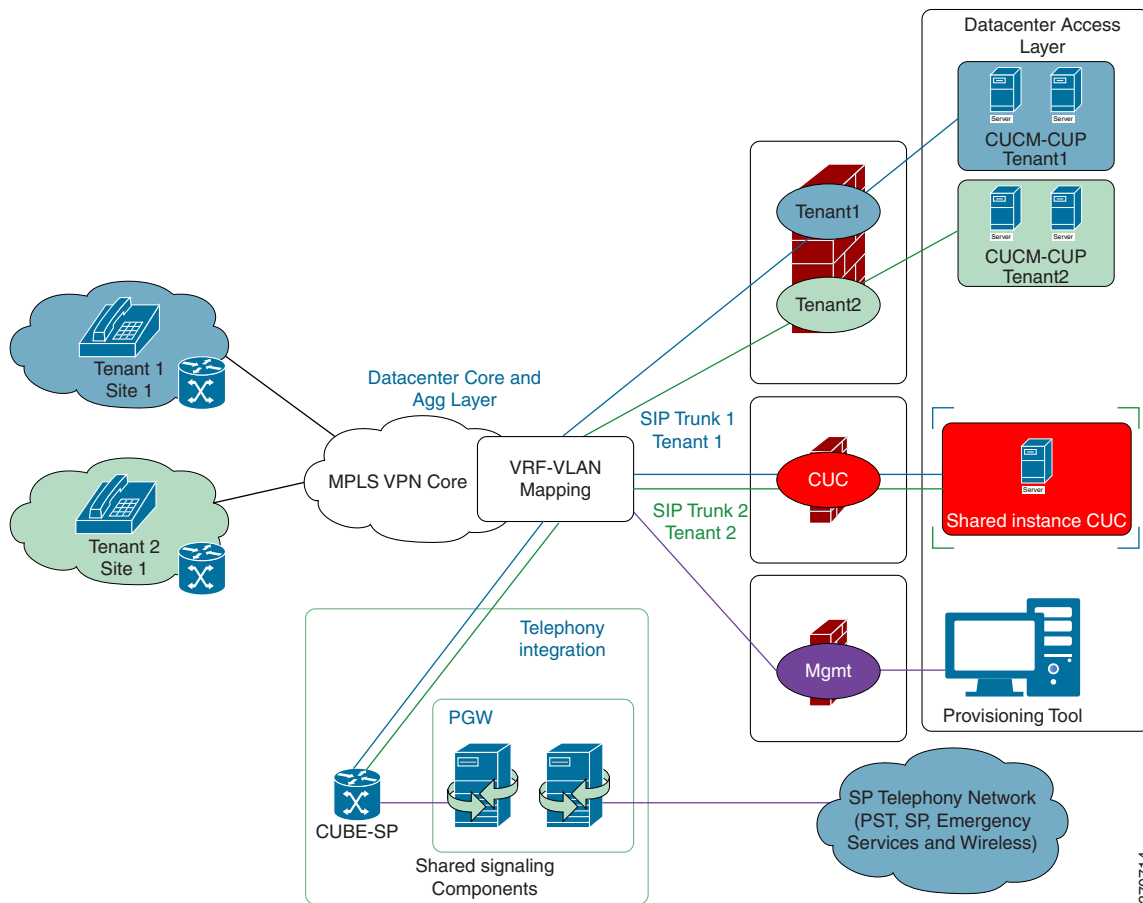
Figure 7-1 Sample Deployment
