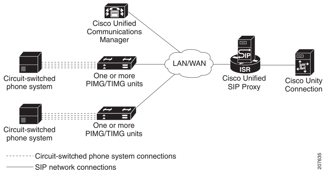
Figure 11-7 Connections for PIMG/TIMG and Cisco Unified Communications Manager Through Cisco Unified SIP Proxy
