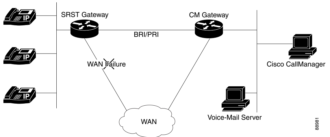
Figure 11-10 Cisco Unified Communications Manager Fallback with BRI or PRI
