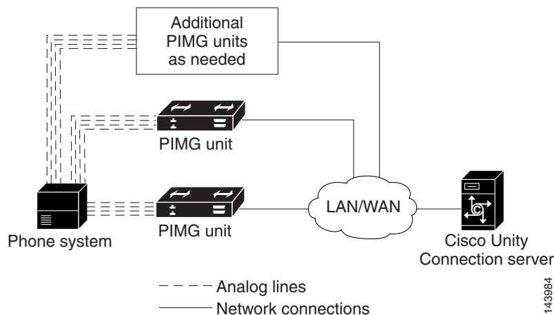
Figure 11-3 Connections for a DTMF Integration Using Analog PIMG Units
