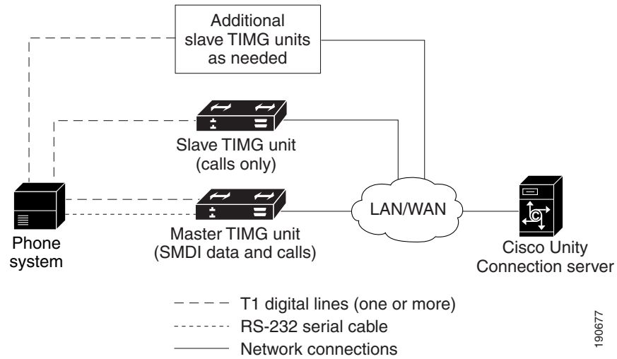
Figure 11-5 Connections for a Serial Integration Using TIMG Units
