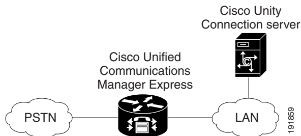
Figure 11-8 Cisco Unity Connection SCCP and SIP Connections to Cisco Unified Communications Manager Express Over a LAN
