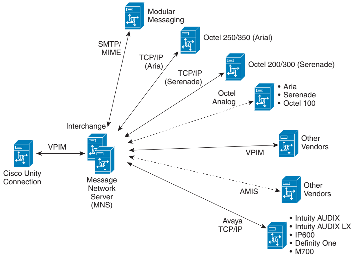
Figure 5-5 Cisco Unity Connection Communicates with the Avaya Message Network Solution
