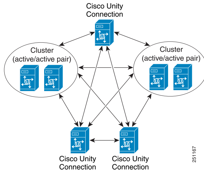
Figure 5-2 A Cisco Unity Connection Site Joined by Intrasite Links Among Locations
