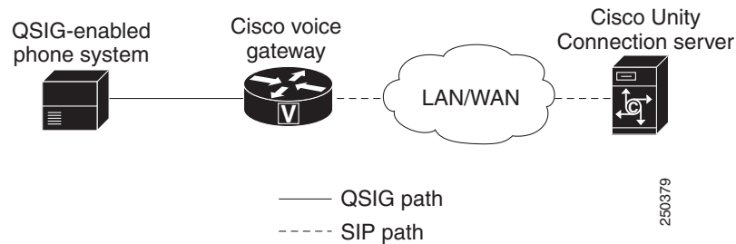
Figure 11-12 Connections Between the Phone System and Cisco Unity Connection
