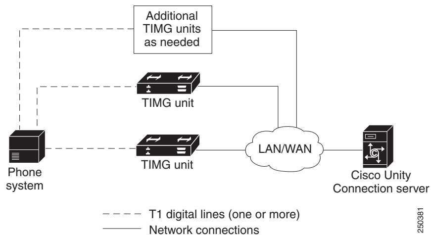
Figure 11-6 Connections for an In-Band Integration Using TIMG Units
