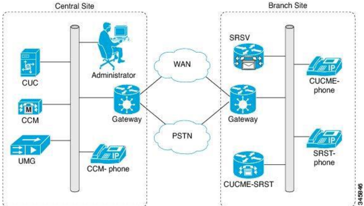
Figure 16-2 Topology 2
