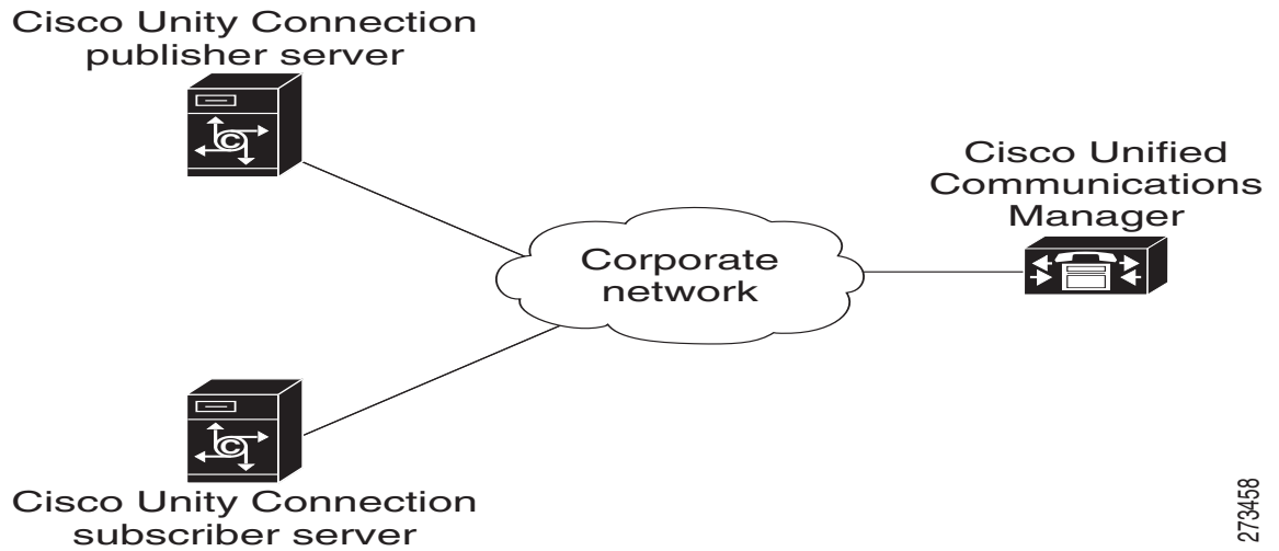
Figure 12-1 Cisco Unity Connection Cluster Integrated with Cisco Unified Communications Manager
