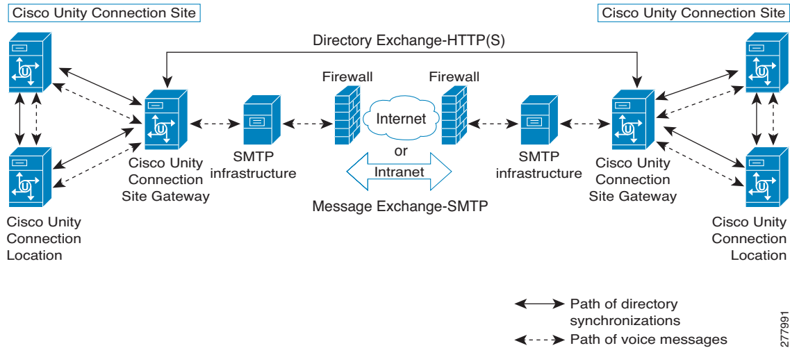
Figure 5-3 Cisco Voicemail Organization Consisting of Two Unity Connection Sites Linked via an Intersite Link
