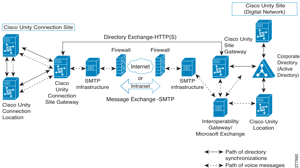
Figure 5-4 Cisco Voicemail Organization Consisting of a Unity Connection Site Linked to a Cisco Unity Site
