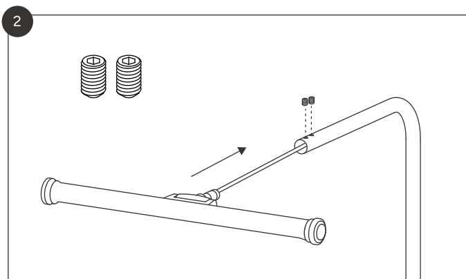
Attach the shade to the stem and insert the upper grub screws to fix in place. Tighten all grub screws.
