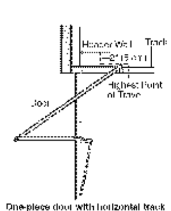
One-piece door with horizontal track
