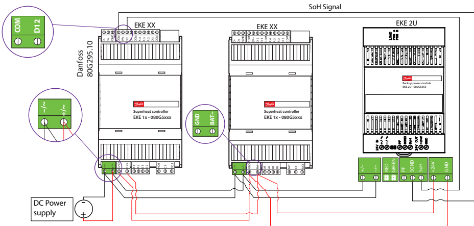
SHARING EKE 2U WITH 2 CONTROLLERS
