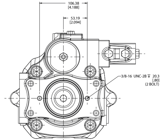
Right hand rotation Shown with Pressure Compensator with Load Sense
