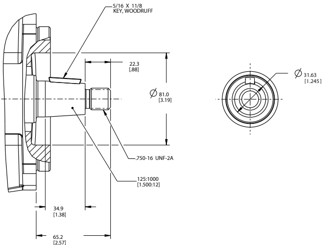
24 - 24 - 31.8 [1.25] DIA TAPERED KEYED SHAFT .750-16 UNF-2A EXTERNAL THREAD KEY INCLUDED
