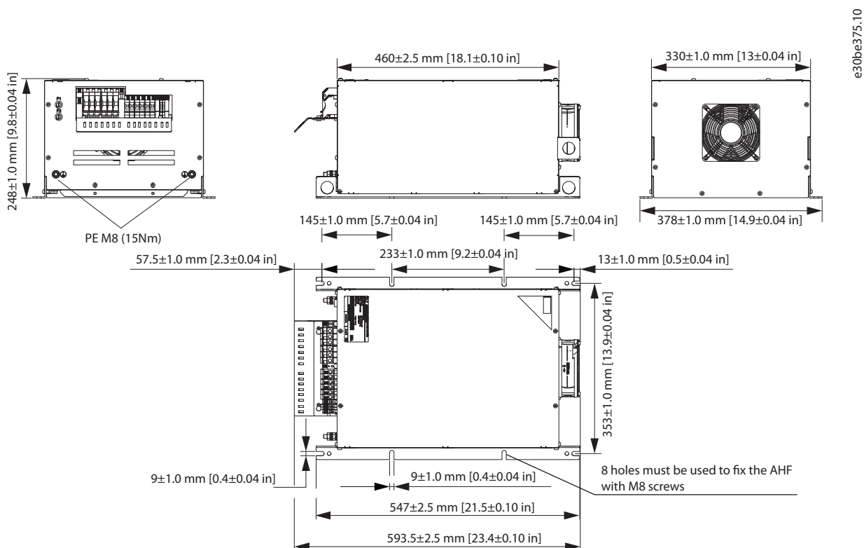
Illustration 7.12 IP20 X3-V3 External Fan
