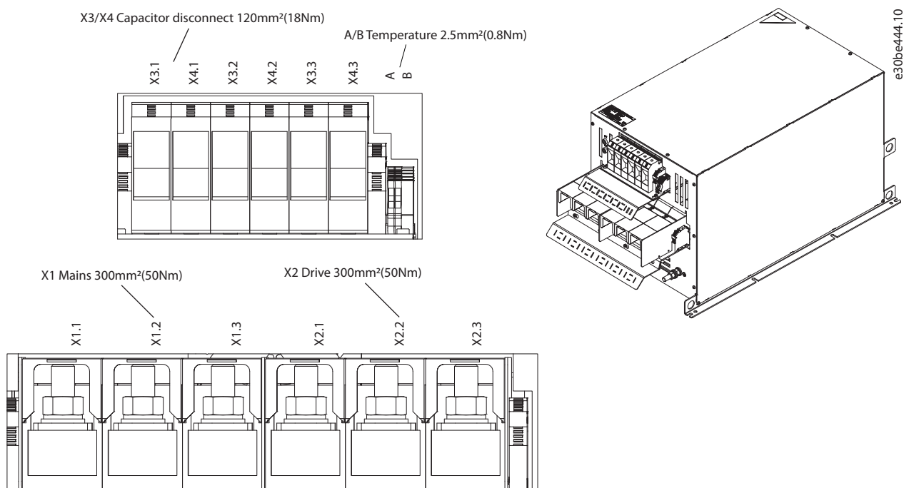
Illustration 7.27 IP20 X7-V3 Internal Fan, Terminal Designation and 3D View
