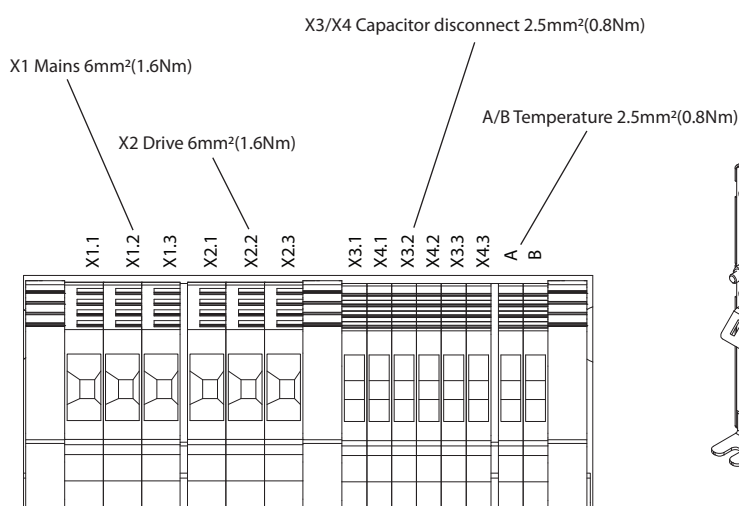
Illustration 7.3 IP20 X1-V3 Internal Fan, Terminal Designation and 3D View
