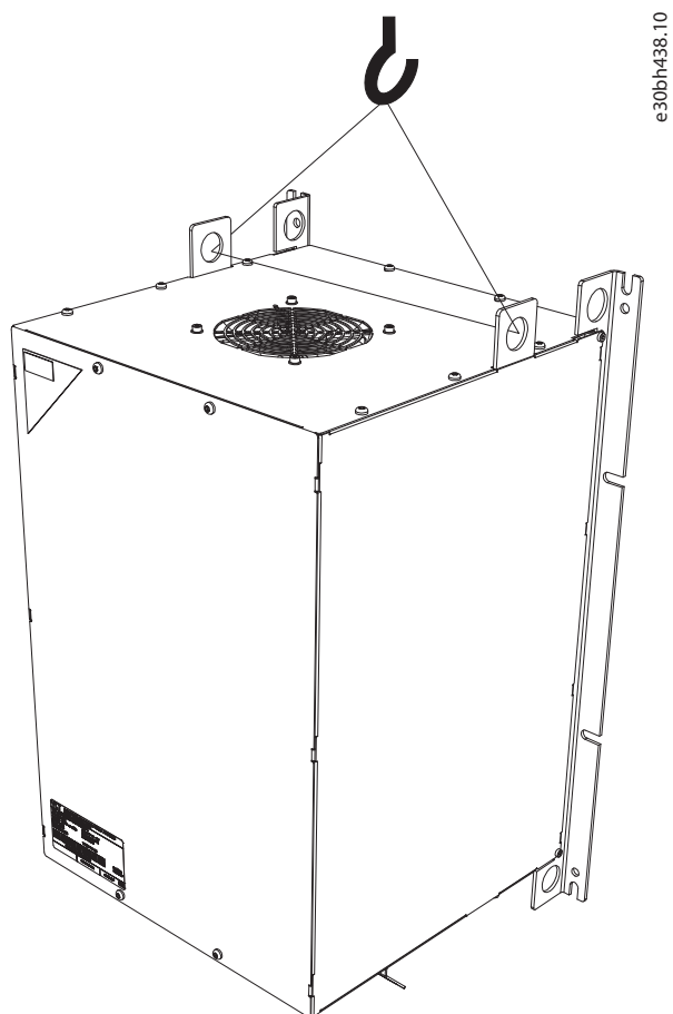
Illustration 4.1 Lifting Method, Internal Fan Filters
