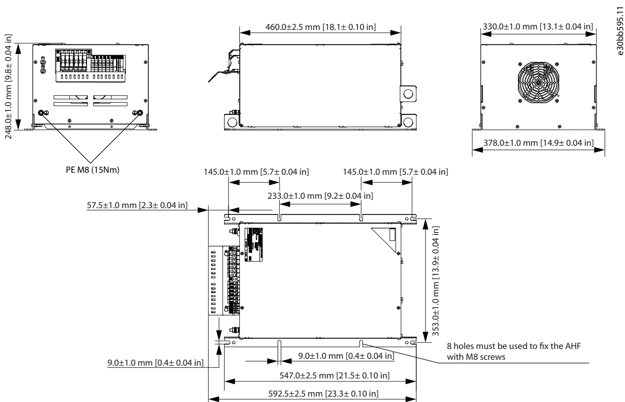
Illustration 7.10 IP20 X3-V3 Internal Fan
