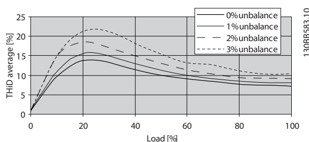
Illustration 3.6 AHF 010
