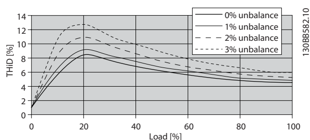
Illustration 3.5 AHF 005
