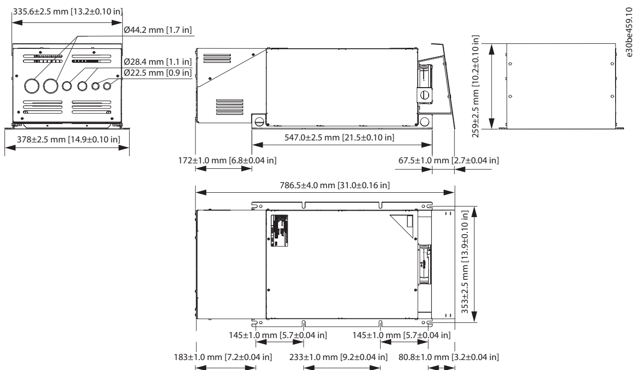
Illustration 7.38 IP21 X3-V3 Internal and External Fan
