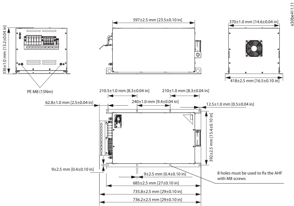
Illustration 7.20 IP20 X5-V3 External Fan
