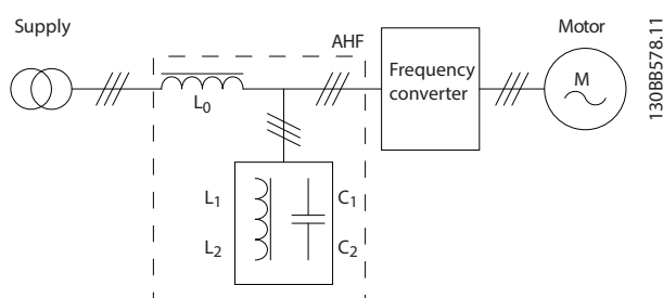
Illustration 3.1 Operating Principle
