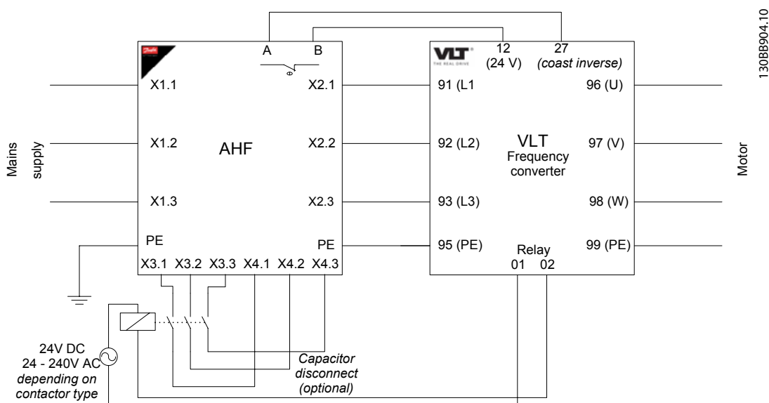
Illustration 4.8 Connection Diagram
