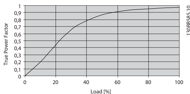
Illustration 3.8 AHF 010
