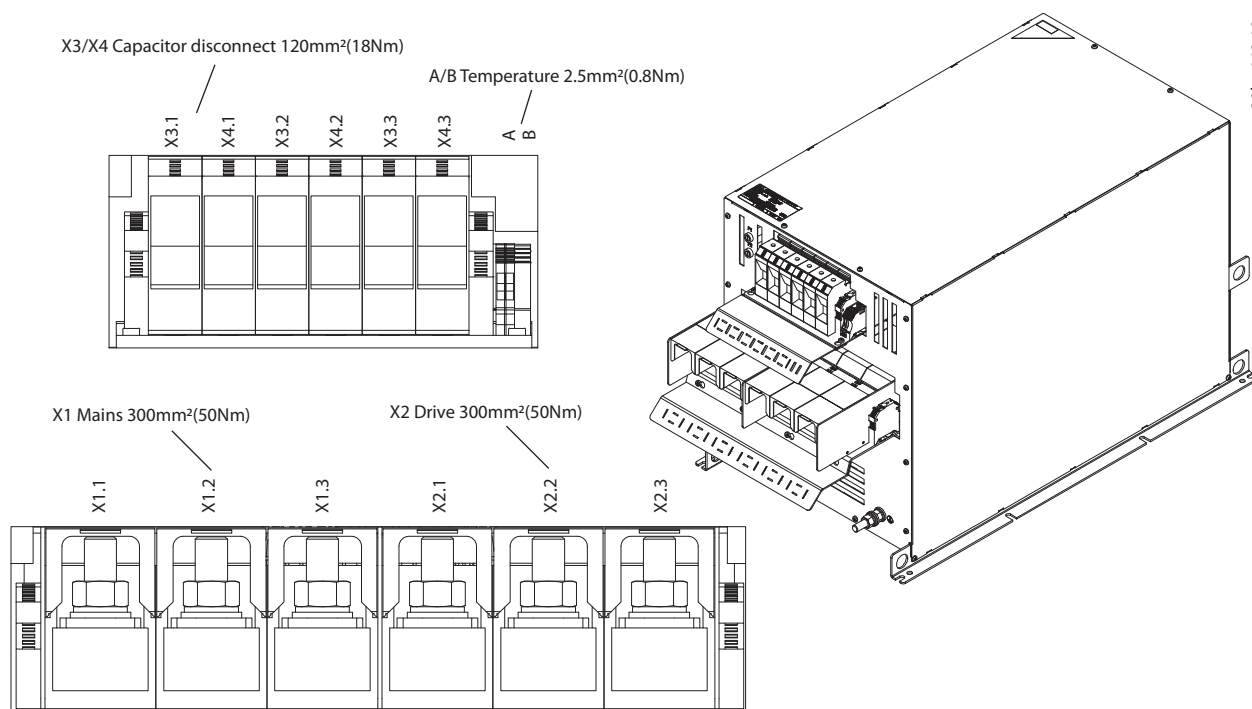
Illustration 7.33 IP20 X8-V3 External Fan, Terminal Designation and 3D View
