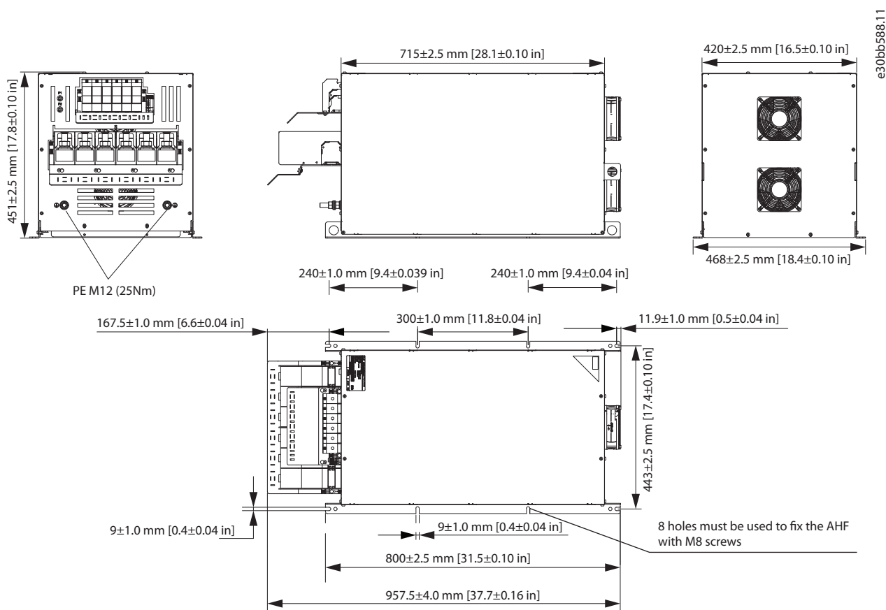
Illustration 7.28 IP20 X7-V3 External Fan
