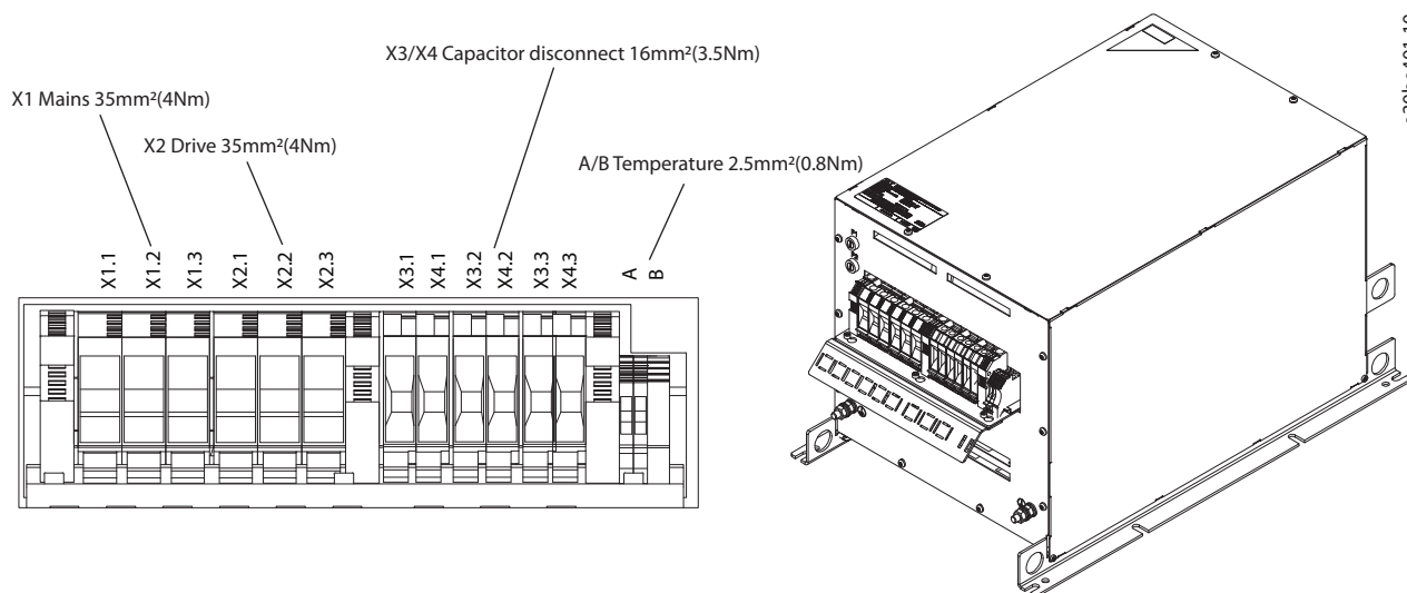
Illustration 7.15 IP20 X4-V3 Internal Fan, Terminal Designation and 3D View
