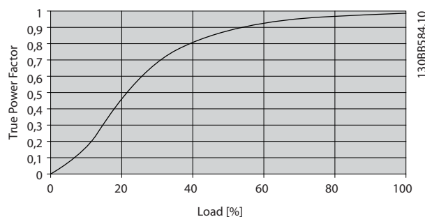
Illustration 3.7 AHF 005
