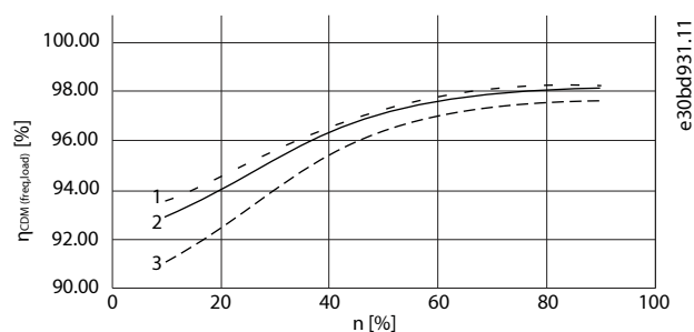
Figure 85: CDM Efficiency ( \eta_{CDM}(\text{freq}, \text{load}) ) [%] versus Speed (n) [% of Nominal Speed]
