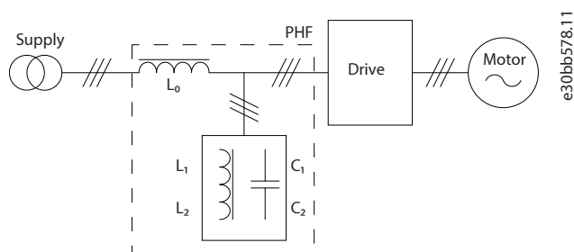
Figure 8: Operating Principle
