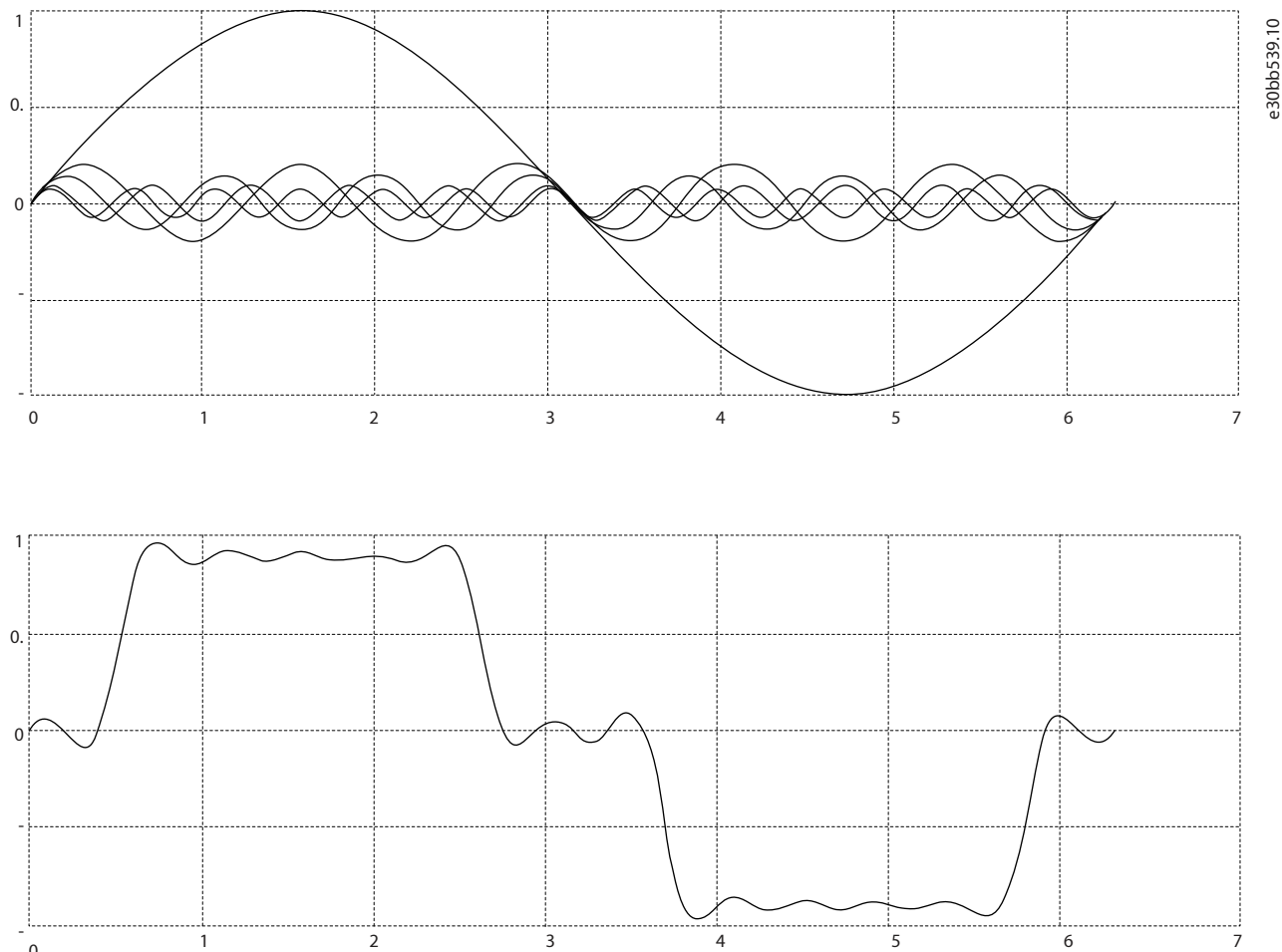
Figure 5: Sinusoidal Waveforms
