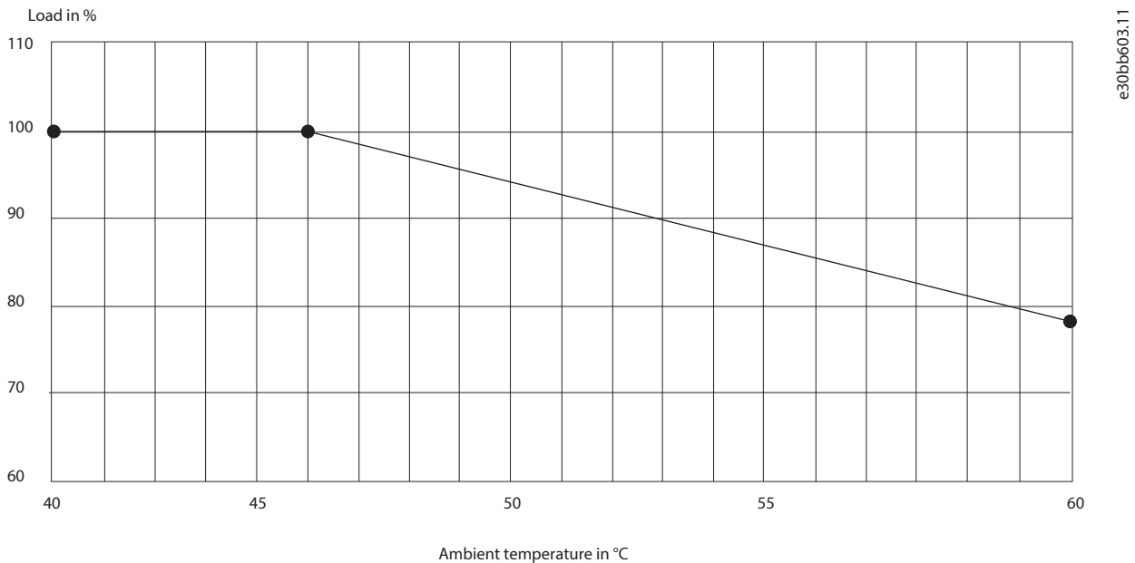
Figure 30: Temperature Derating Curve
