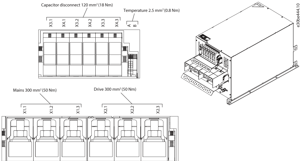
Figure 56: IP20 X7-V3 Internal Fan, Terminal Designation and 3D View
