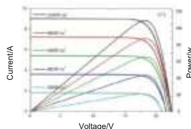
P-V Curves of PV Module(120W)
