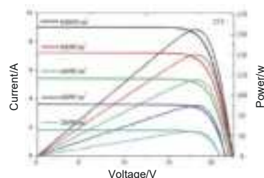
P-V Curves of PV Module(170W)
