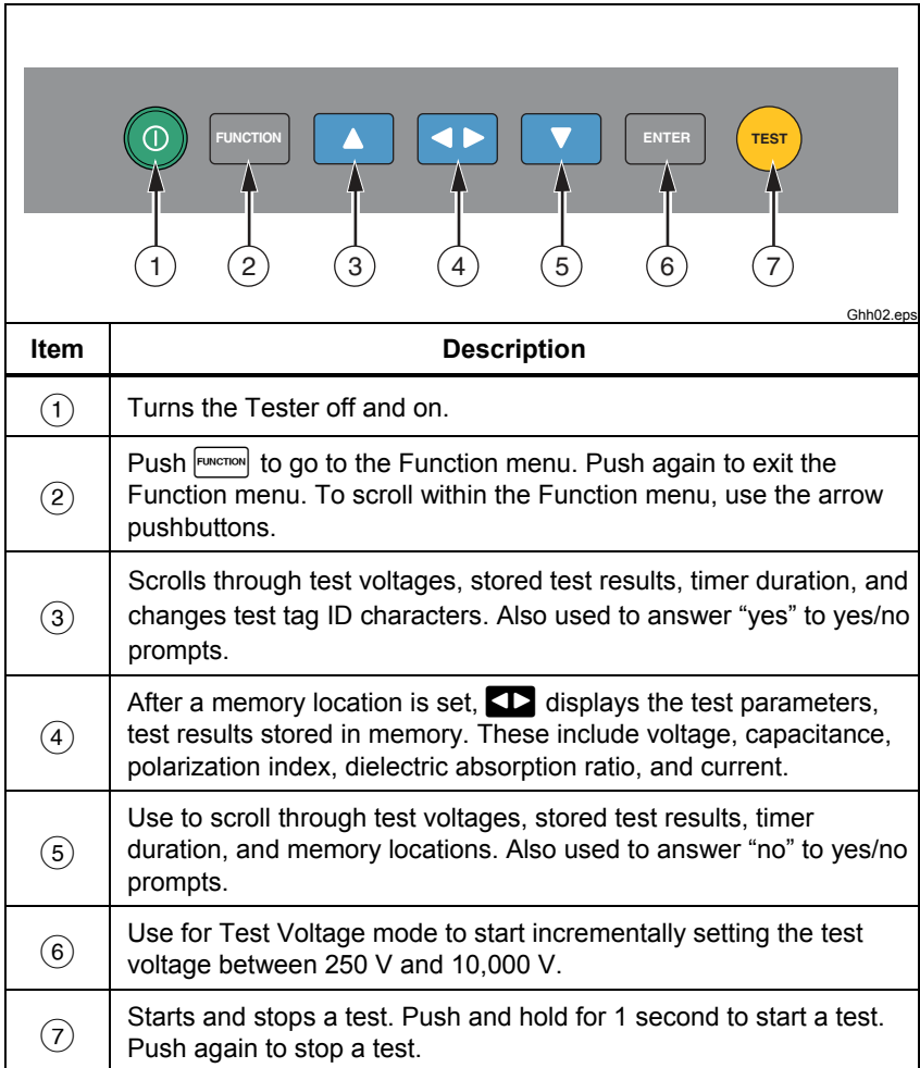
Figure 3. Pushbuttons
