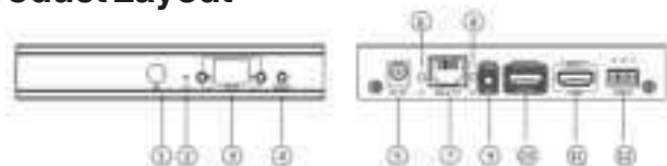
Figure 1: Transmitter (TX)
