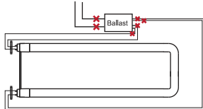
Diagram 5 – Cut all ballast wires
