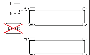
Diagram 4 – Multiple tube wiring
