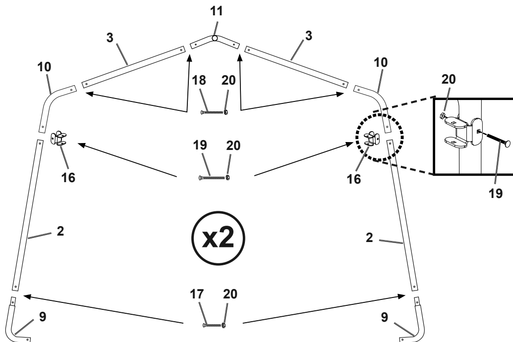
Figure A: End Assembly
