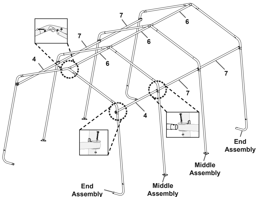
Figure C: Frame Assembly
