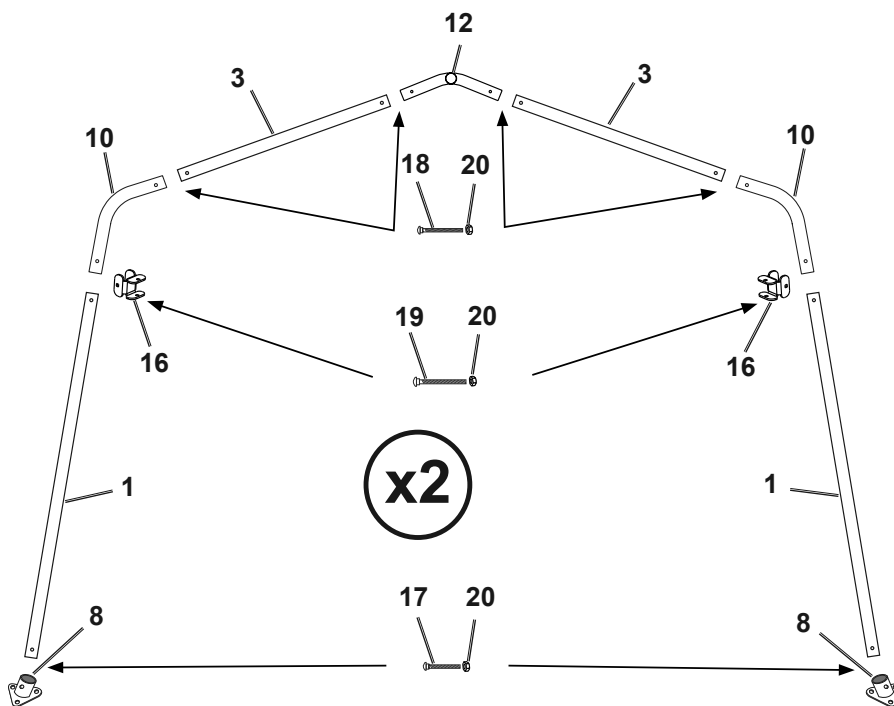
Figure B: Middle Assembly
