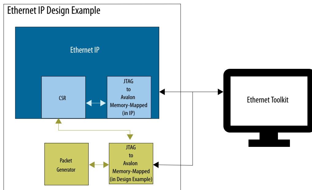
Figure 9. Block Diagram of the Ethernet Toolkit
