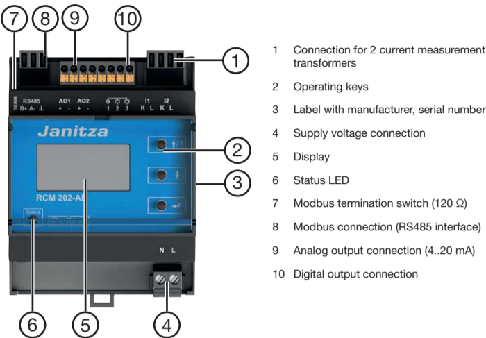
Fig. 1: RCM 202-AB device view
