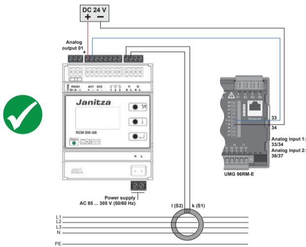
Fig. 7: Connection to the analogue inputs of a UMG 96RM-E
