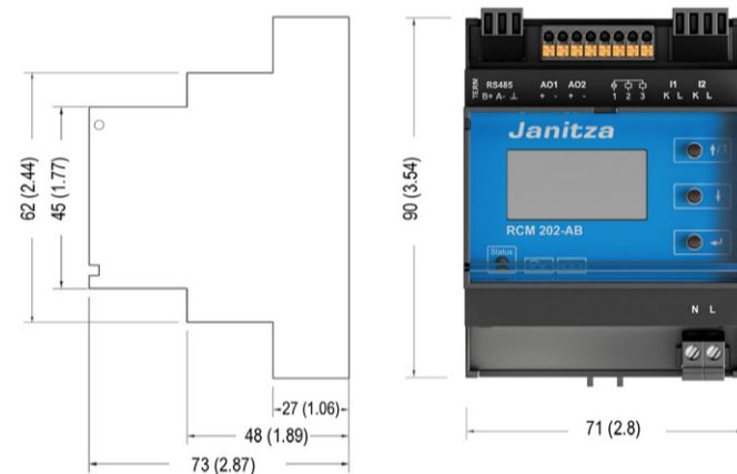
Fig. 2: Device dimensions in mm (in)
