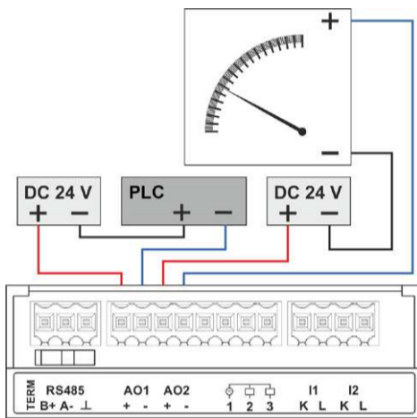
Fig. 6: Connection of a display device and a PLC to the analog outputs (Power supply: Janitza power supply unit, art. no. 16.05.012)
