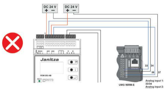
Fig. 8: Invalid connection scheme
