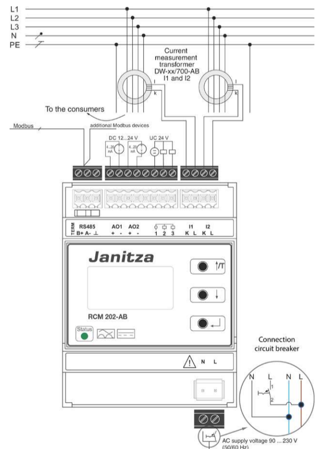
Fig. 4: Circuit diagram of the RCM 202-AB
