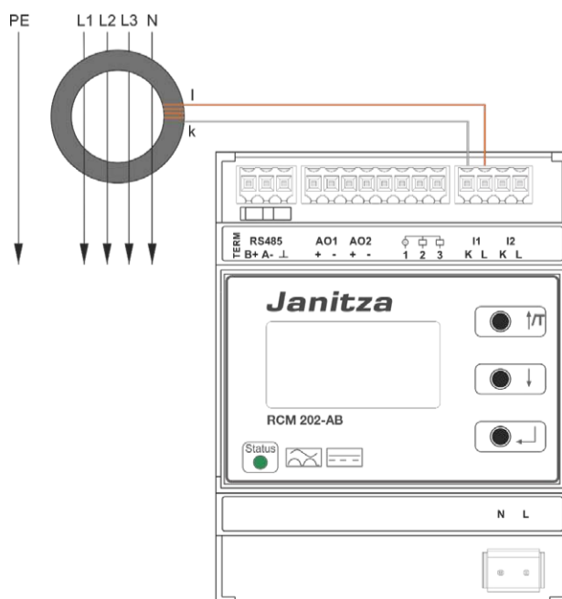
Fig. 3: Simplified presentation of residual current measurement
