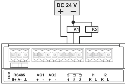
Fig. 5: Connection of two relays to the digital outputs
