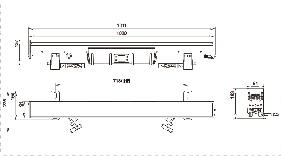
Size-Fig.2(Unit: mm)
