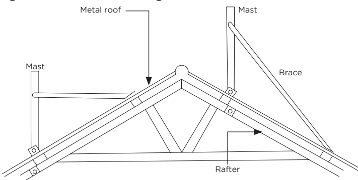
Fig. 2 Alternate brace arrangements for Metal Roofs
