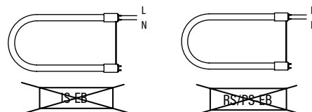
STEP B - The wiring can be single end or double end. Refer to Fig. 3.
