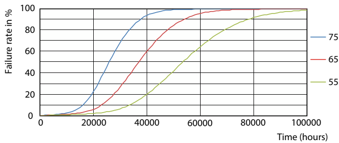
Life Expectancy Diagram - 12T8/COR/48-5CCT/FF18/G/DIM 25/1
