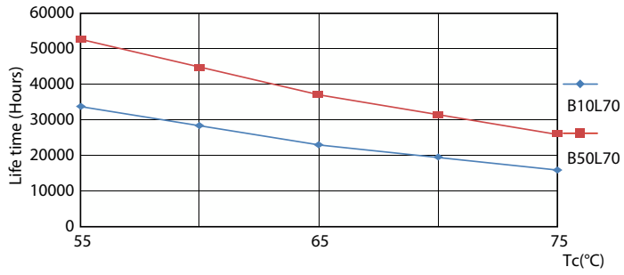
Life Expectancy Diagram - 12T8/COR/48-5CCT/FF18/G/DIM 25/1
