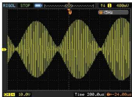
Figure 9 — Two-tone RF-modulated transceiver output measurement with the Rigol DS1052E using the same test setup as for Figures 4 and 5.
