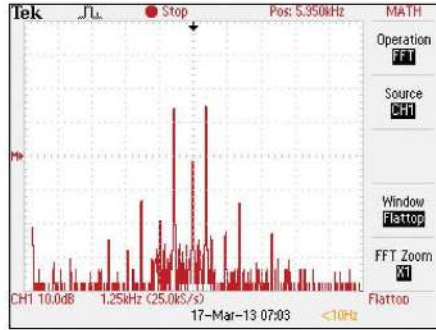
Figure 5 — Tektronix TBS1042 two-tone test FFT display using the same test setup as for Figure 4.
