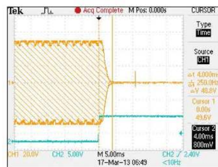
Figure 3 — Transceiver un-key/RF output timing measurement with the Tektronix TBS1042.
