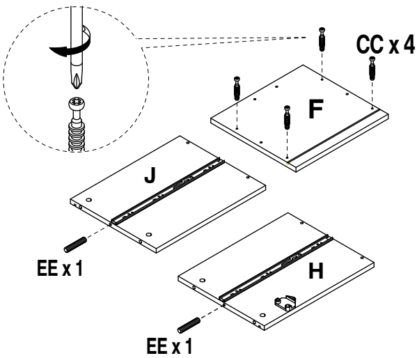
a) Drawer front and upper drawer right preparation
