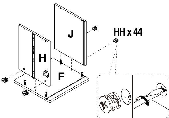
b) Attaching drawer sides
