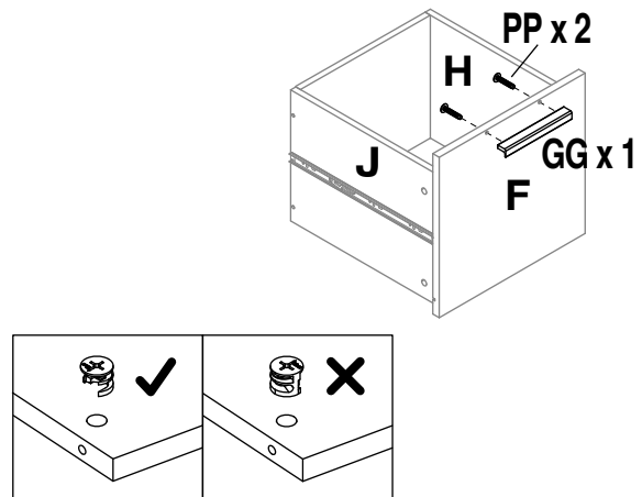
d) Attaching handle
