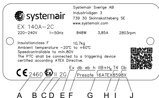
Fig. 4 Name plate
