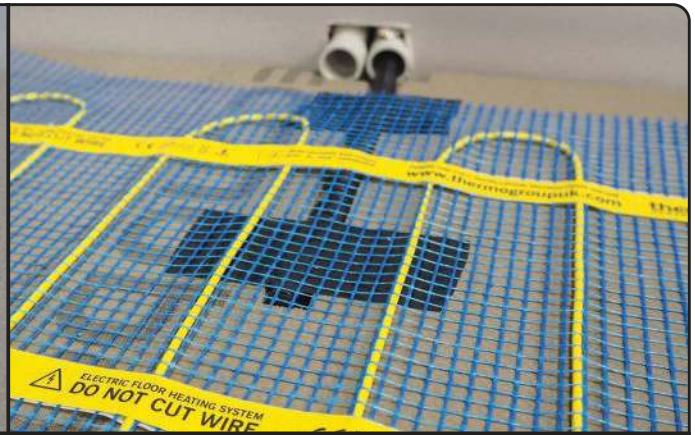
Ensure the floor sensor conduit is located evenly between two runs of heating cable.
