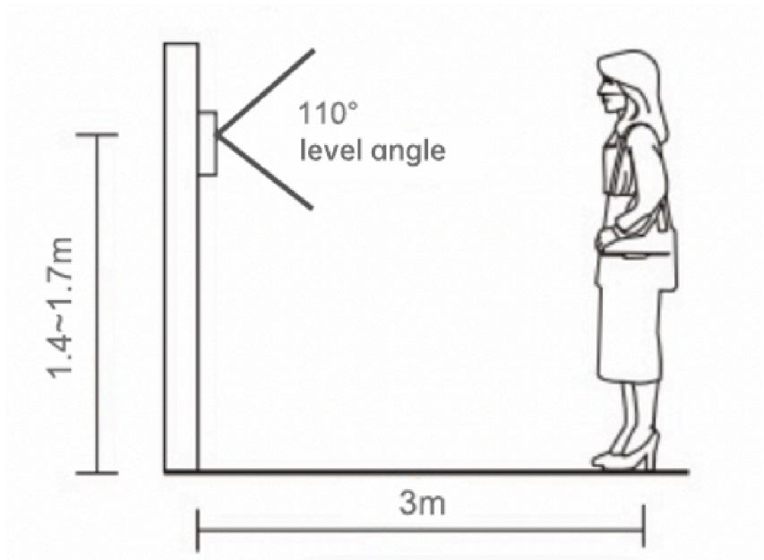
Image 1-1 Outdoor Station Installation Diagram
