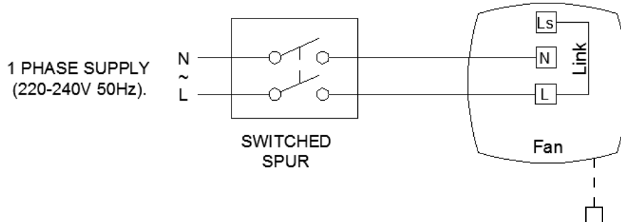
Fig.3. Continuous trickle with boost facility. (The fan is internally fused)
