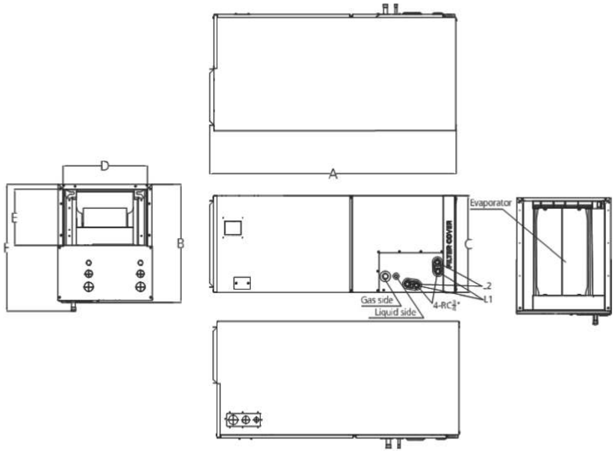
Fig. 8 —Dimensions
