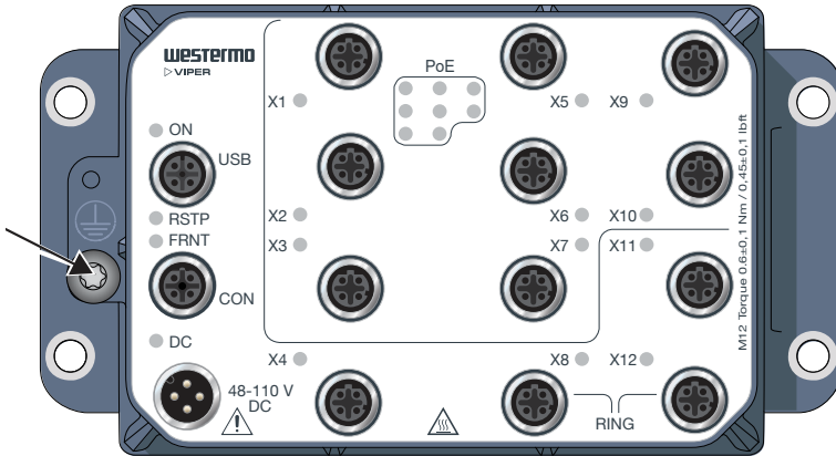
Figure 6. Earth connection
