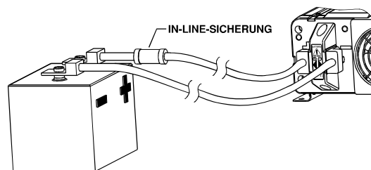
Abb. 4. Batterieanschlüsse
