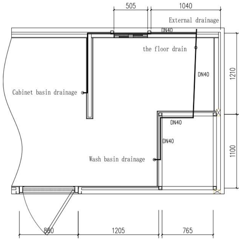
Drainage layout plan
