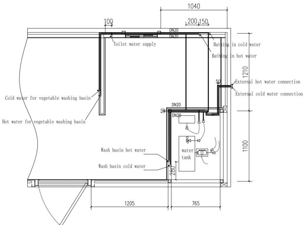
Layout of cold and hot horizontal planes
